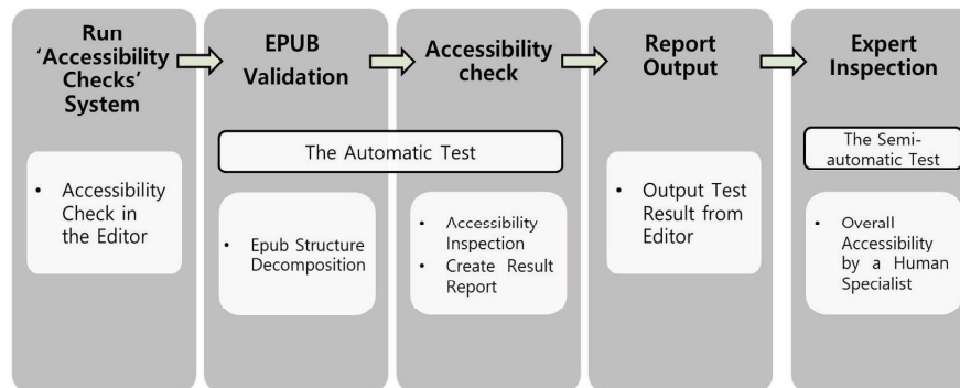
Fig. 3. Overall System Process.
